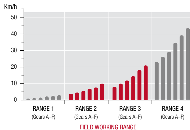
DYNA-6 TRANSMISSION
